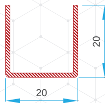
Screen Sash Reinforcement 56016 - 15501
