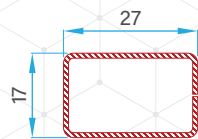
Frame Profile / Mullion Profile 56016 - 10043
