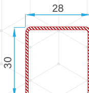
Large Frame Profile 56016 - 10057
