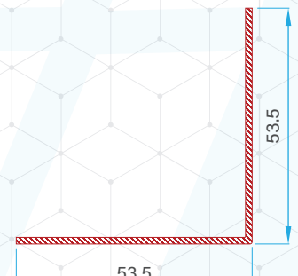
Corner Profile - 90° 56016 - 15050
