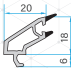
Single Glazing Bead (6mm) 77390-20710
