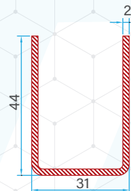
Mega Sash Reinforcement 56016 - 20207
