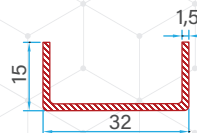
Sash Reinforcement 56016 - 15187
