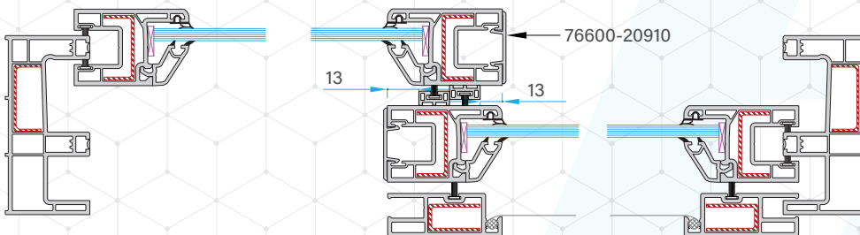
SEC-BB
