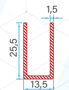
Screen Sash Reinforcement 56016 - 15078
