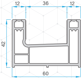
Double Rail Profile 76601-10110
