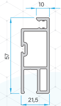
Screen Sash (P-60) 76601-10710
