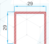
Super Sash Profile (P-55) Reinforcement 1.5mm : 56016 - 15167
